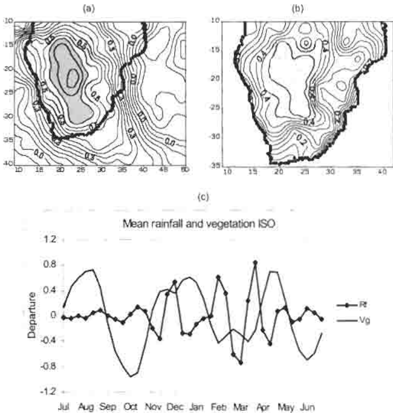
Fig. 6.3 Intraseasonal spatial loadings for (a) rainfall PC1 and (b) NDVI PC1 for the 40-days oscillation and (c) the seasonal mean ISOs.
