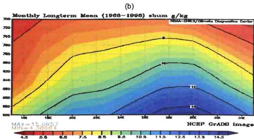
Fig. 1.4. (a) Vertical profile of the planetary boundary layer (after Stull, 1988) (b) Long term mean distribution of specific humidity over southern Africa plotted as an east-west cross section from the plateau upward to 3 km elevation, averaged for latitude 27°S.
