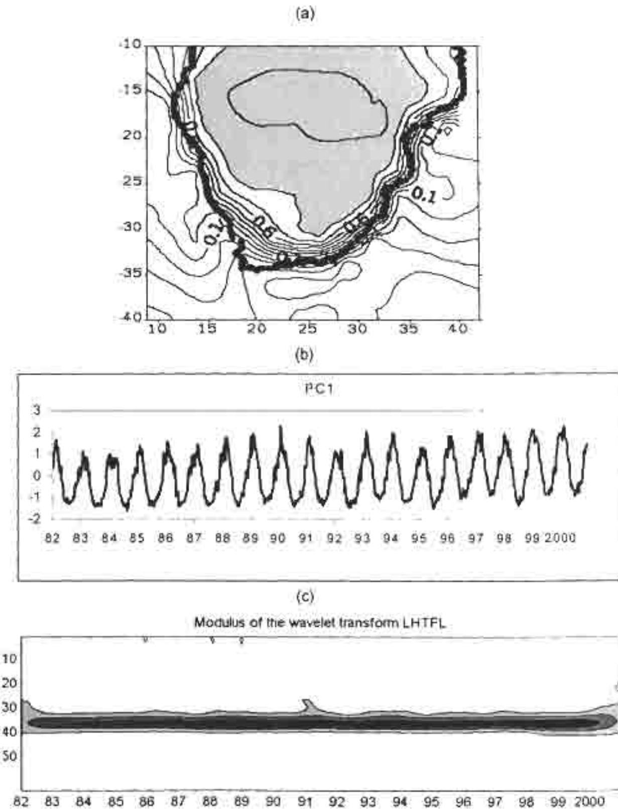
Fig 5 4 (a) Spatial loadings (b) time scores and (c) modulus spectrum for NCEP model latent heat flux (unfiltered and unrotated) seasonal cycles (PC1) over southern Africa.
