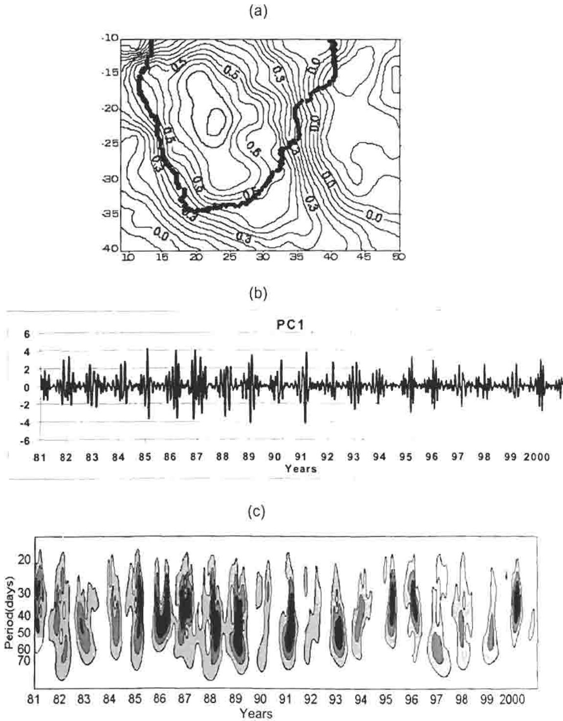
Fig. 3.3. (a) Spatial loading (b) the associated time scores and (c) the modulus spectrum for Intra-seasonal rainfall (filtered to retain cycles between 20-70days and unrotated) for PC1.
