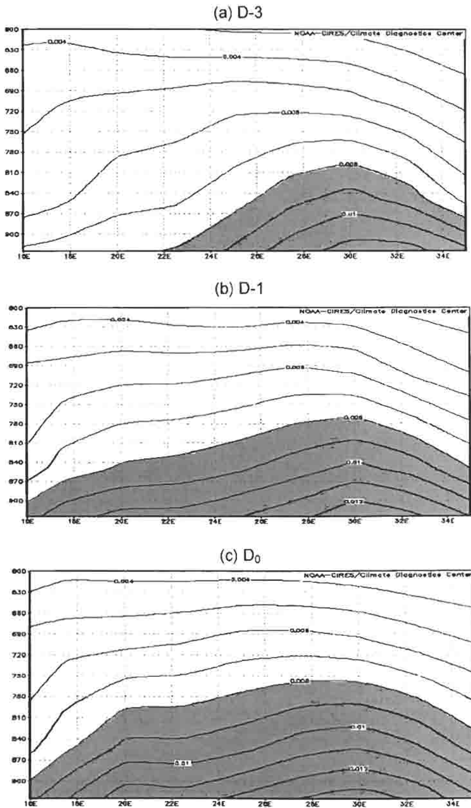
Fig. 6.7 Dekad mean composite NCEP specific humidity in the boundary layer from 925 hPa to 600 hPa averaged from 17°S to 27°S and from 16°E to 35°E, for NDVI 'big' event cases. The layer > 0.008 g/kg is shaded.
