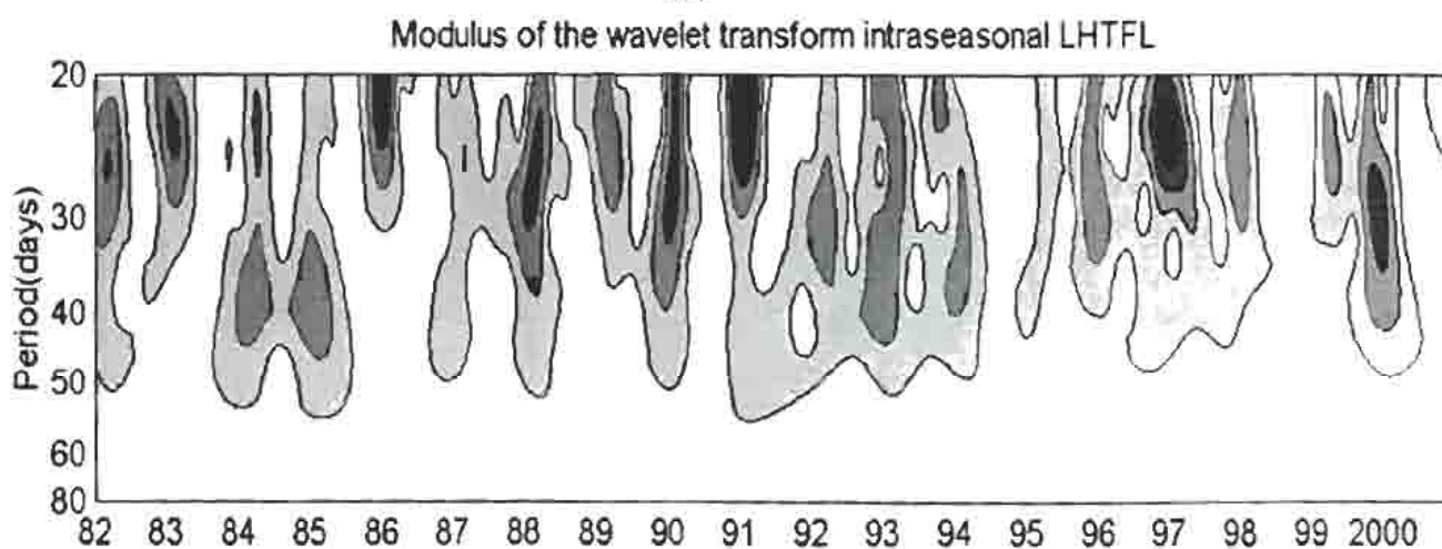
Fig. 5.6 (a) Spatial loadings (b) time scores and (c) modulus spectrum for intraseasonal NCEP model latent heat flux (filtered and rotated) PC2 over southern Africa.
