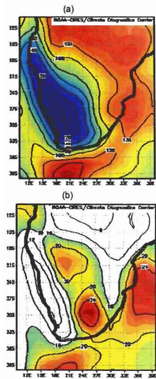
Fig. 5.3 (a) DJF NCEP model latent heat flux climatology (1968-1996) and (b) the interannual standard deviation (1982-2000)
