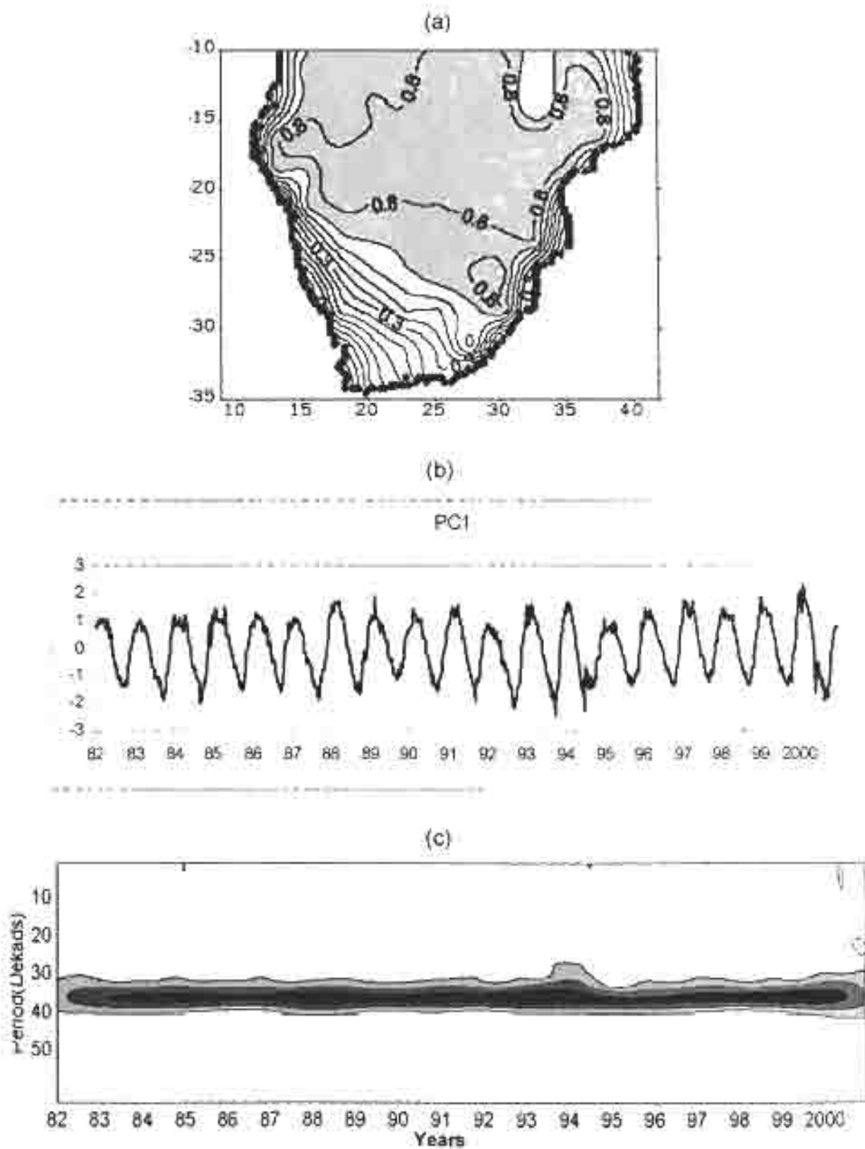
Fig. 4.5 (a) Spatial loading and (b) the associated time scores and (c) the modulus spectrum for seasonal vegetation NDVI (unfiltered and unrotated) for PC1 accounting for 34% of total variance.
