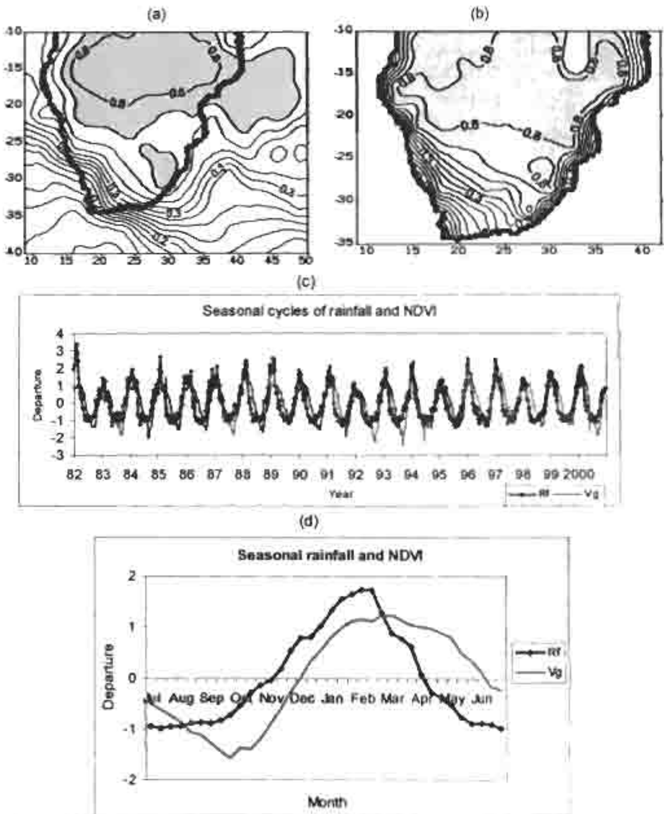
Fig. 6.2 Seasonal spatial loadings for (a) rainfall and (b) NDVI (c) the associated time scores showing pronounced cycles and (d) the seasonal mean.
