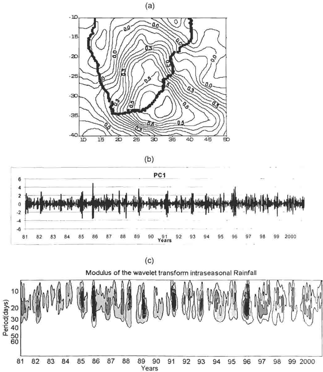
Fig. 3.4. (a) Spatial loading (b) the associated time scores and (c) the modulus spectrum for Intra-seasonal rainfall (filtered to retain cycles between 10-35 days and rotated) for PC1.
