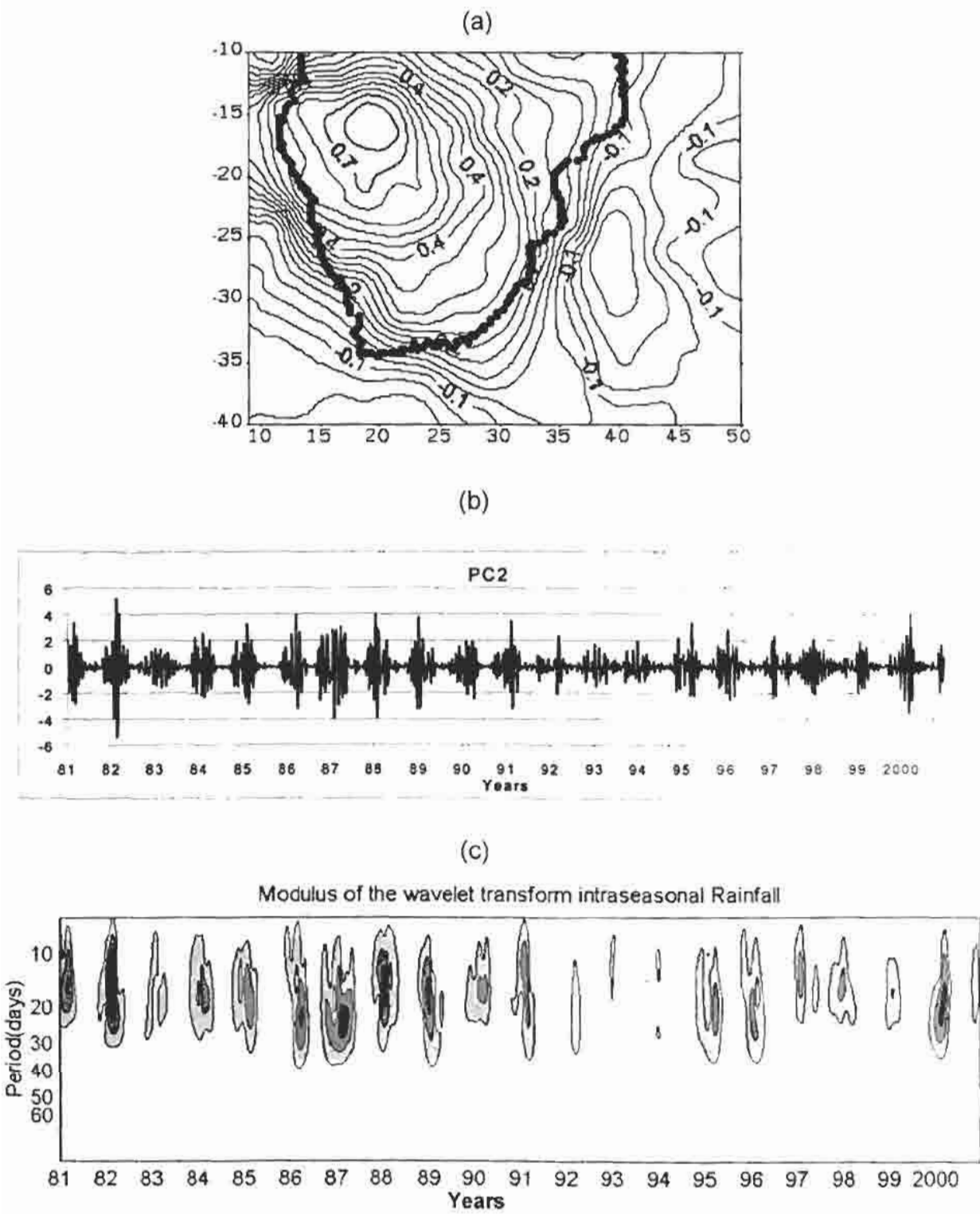
Fig. 3.5. (a) Spatial loading (b) the associated time scores and (c) the modulus spectrum for Intra-seasonal rainfall (filtered to retain cycles between 10-35 days and rotated) for PC2.
