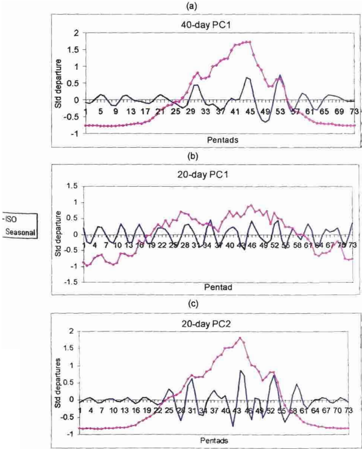
Fig. 3.8 Intraseasonal cycles of rainfall for (a) 40-day Kalahari PC1 (b) 20-day Agulhas PC1 and (c) 20-day Angola PC2 compared against climatology averaged over 20 years (1981-2000). Pentad 1 refers to 30 June to 4 July and pentad 73 refers to 25-29 June.
