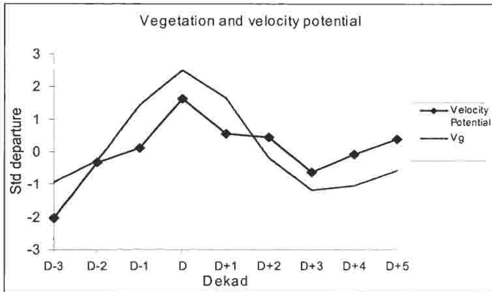
Fig. 6.9 Composite analysis of satellite vegetation and NCEP model low level velocity potential.
